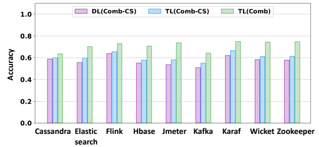
Figure 9: The accuracy of log level suggestions across systems. CS indicates Cross-System.
